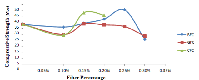
Fig. 1 Variation of 7-Days Compressive Strength for Different SCC Mixes
